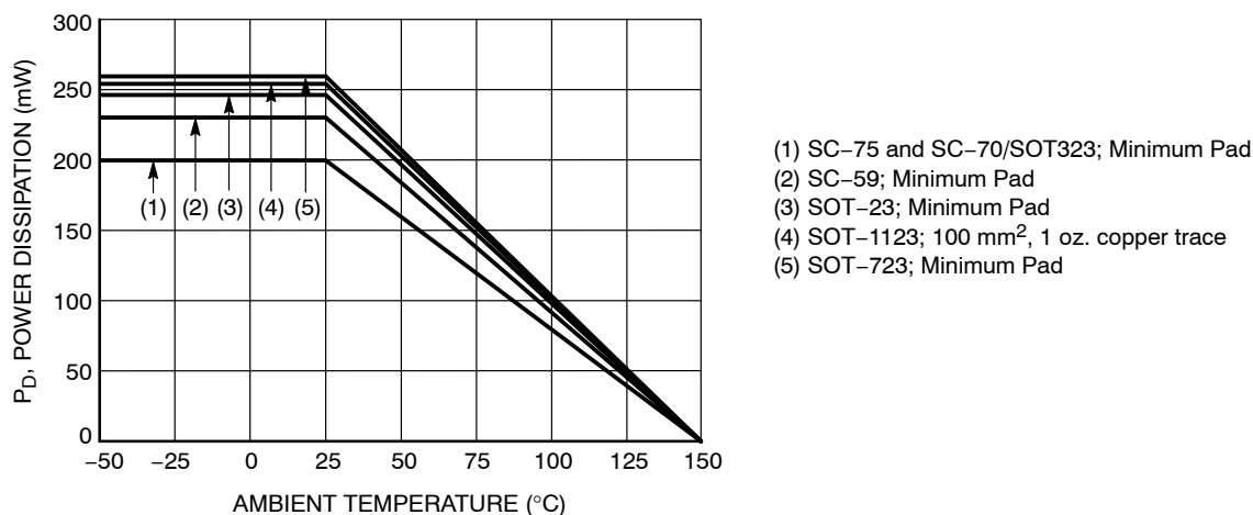
Figure 1. Derating Curve
