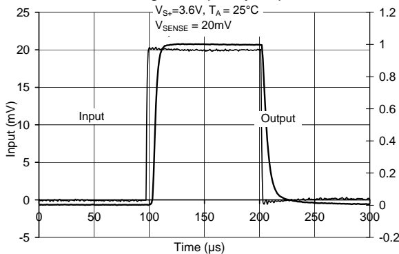
Large signal pulse response 20mV
