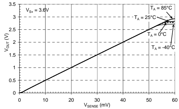
Output Voltage Vs Sense voltage
