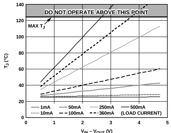
Figure 34. 700 mm 2 of PCB Copper, T_A = 25^\circ\text{C}
