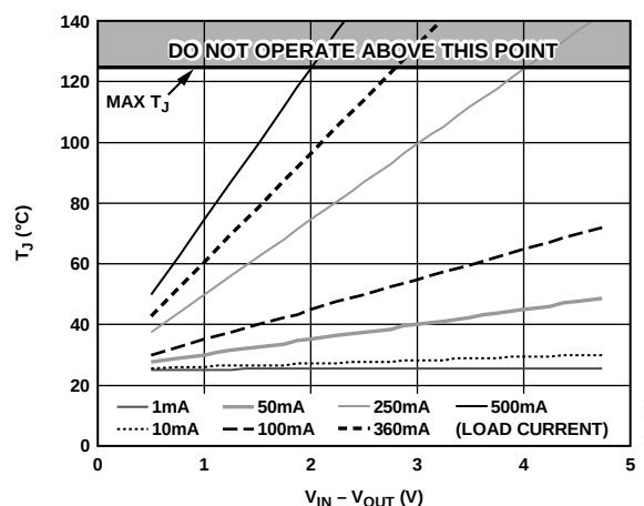
Figure 36. 100 mm 2 of PCB Copper, T_A = 25^\circ\text{C}
