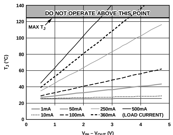
Figure 35. 300 mm 2 of PCB Copper, T_A = 25^\circ\text{C}
