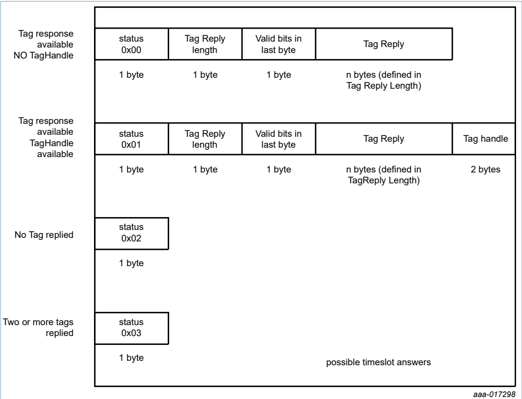
Figure 26. EPC GEN2 possible timeslot answers
