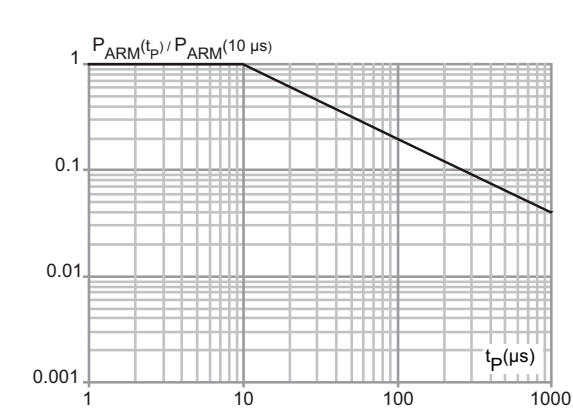
Figure 3. Normalized avalanche power deratings versus pulse duration ( T_j = 125^\circ\text{C} )
