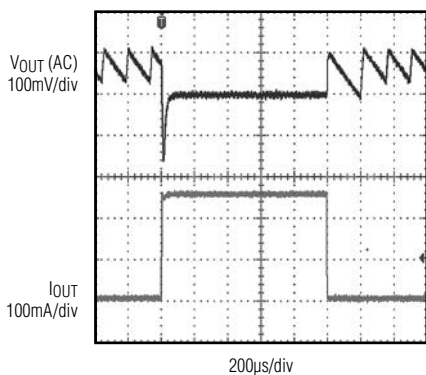
Figure 6. MAX17501A 5mA to 255mA Load Transient
