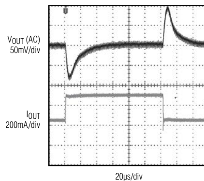
Figure 8. MAX17501A/MAX17501E 250mA to 500mA Load Transient
