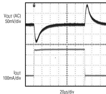
Figure 7. MAX17501E No Load to 250mA Load Transient
