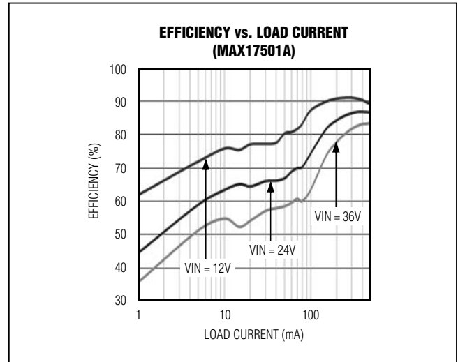
Figure 3. MAX17501A Efficiency
