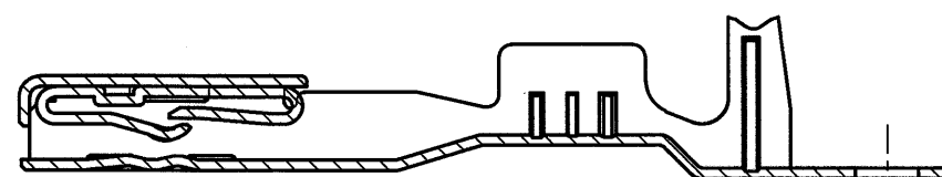
SECT. B-B (SCALE 5:1)
