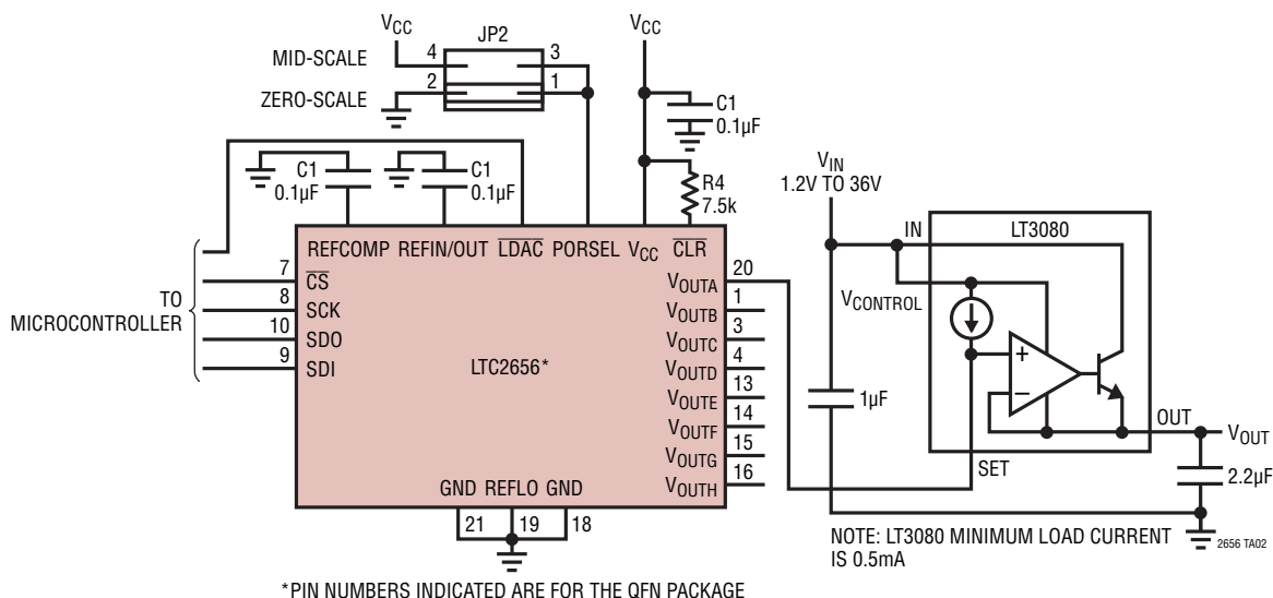
Digitally Controlled Output Voltage 1.1A Supply
