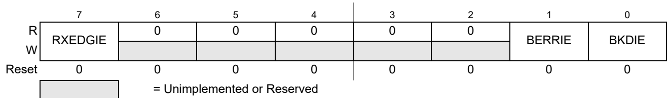
Figure 18-7. SCI Alternative Control Register 1 (SCIACR1)
