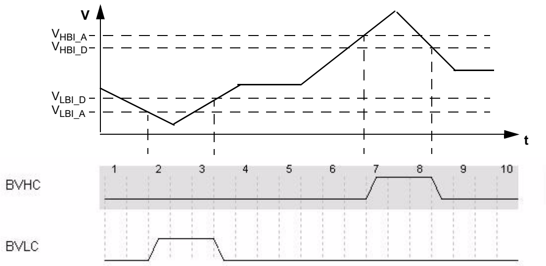
Figure 14-5. BATS Voltage Sensing
