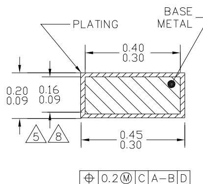
SECTION F-F ROTATED 90°CW 32 PLACES
