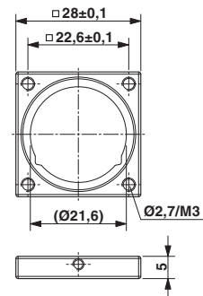
Dimensioned drawing
