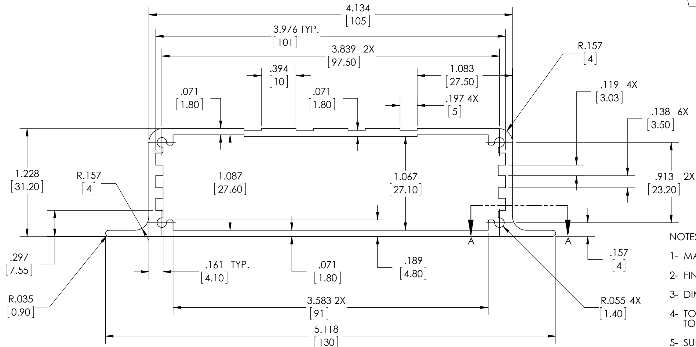
EXTRUSION PROFILE
