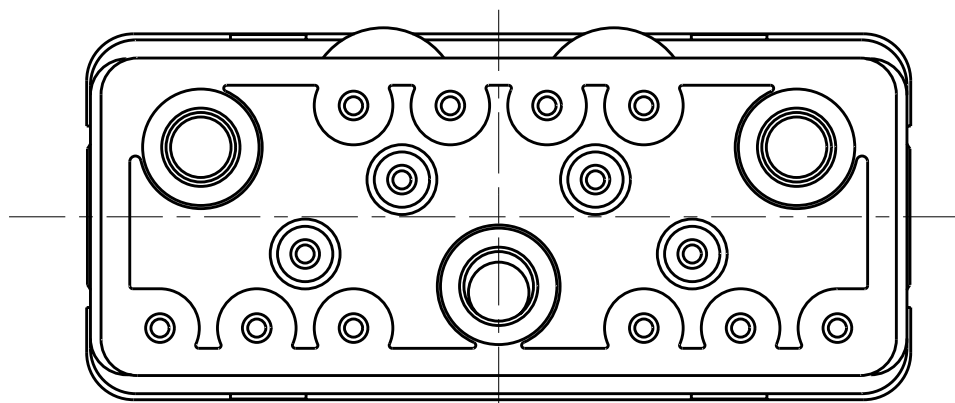
MATING FACE
