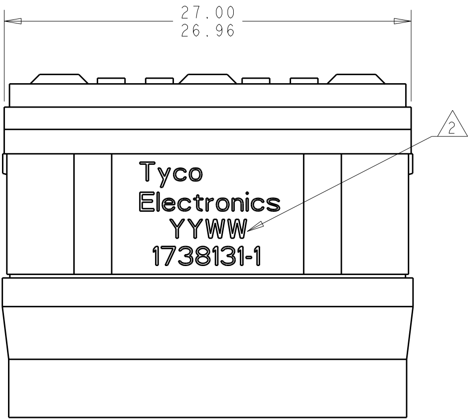
MATING FACE
