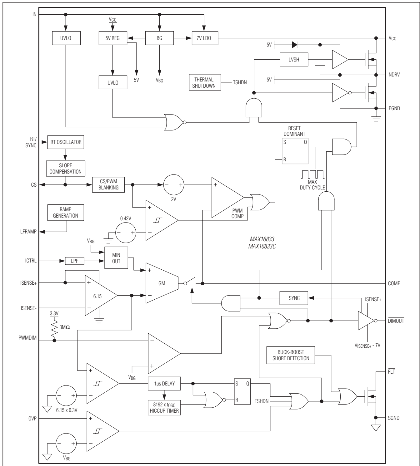
MAX16833/MAX16833C Functional Diagram
