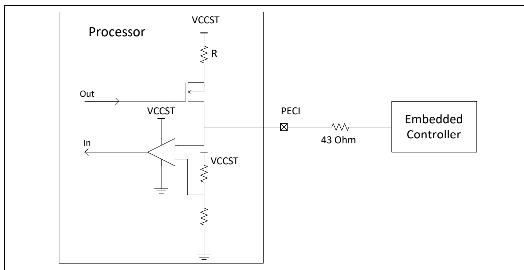
Figure 2-11. Example for PECEC Connection
