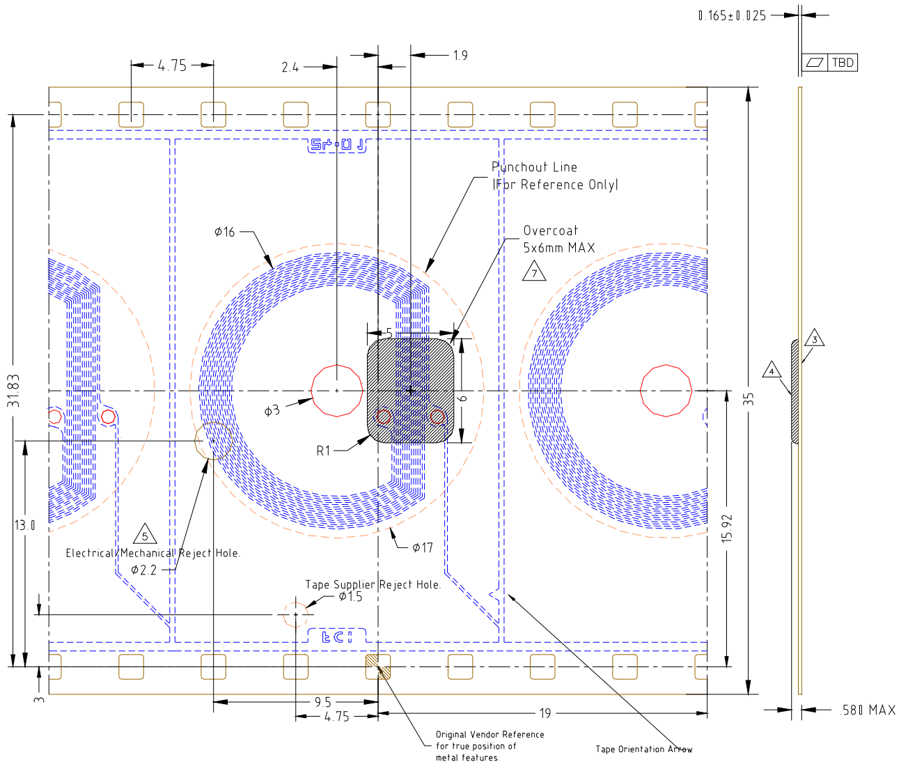
Figure 3. AT88RF04C-MY1G and AT88SCxxxxCRF-MY1
