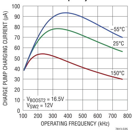
BOOST2 Charge Pump Charging Current vs Frequency
