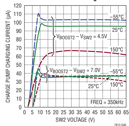
BOOST2 Charge Pump Charging Current vs Switch Voltage
