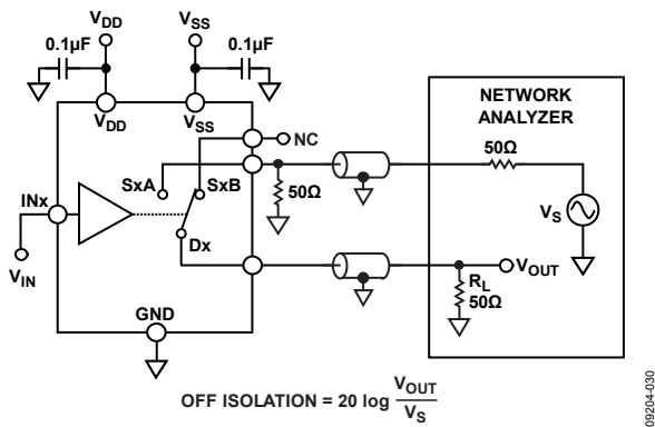
Figure 27. Off Isolation
