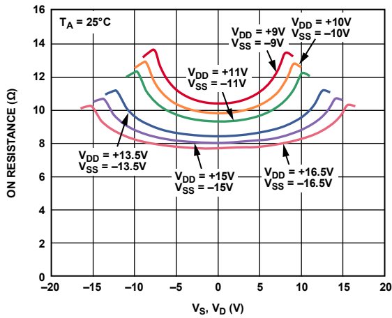
Figure 5. On Resistance vs. V_S , V_D (Dual Supply)
