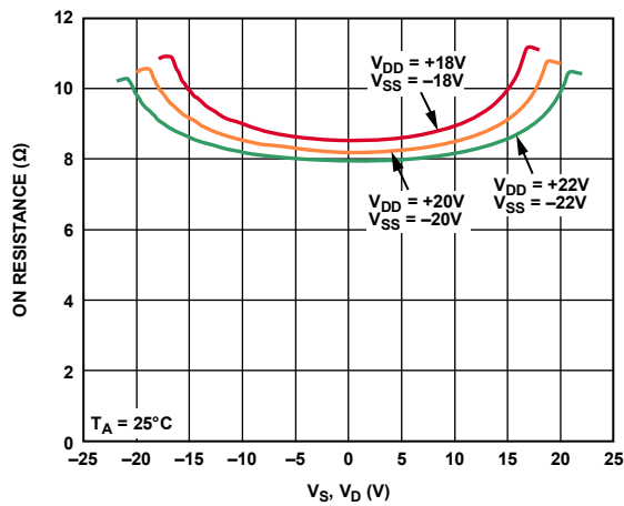
Figure 6. On Resistance vs. V_S , V_D (Dual Supply) Included
