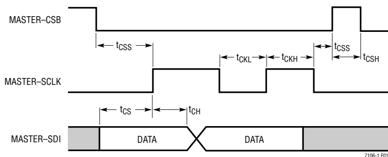
Figure 1. Serial Port Write Timing Diagram
