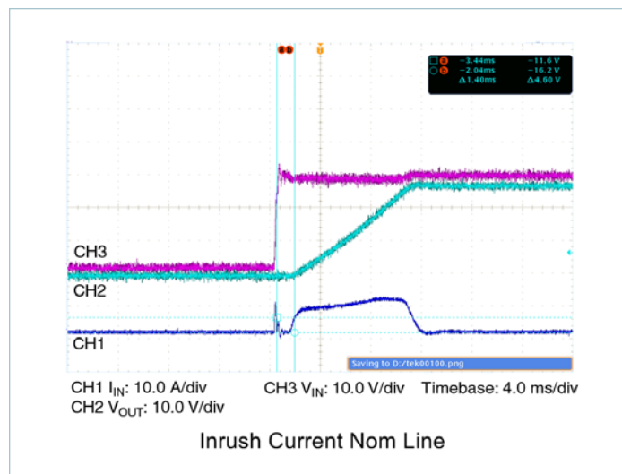
Figure 4 — Inrush limiting; inrush current with 3300 \mu F external capacitance
