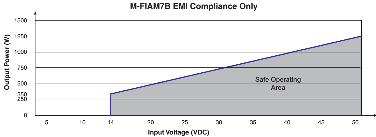
Figure 6 — M-FIAM7B EMI compliance only
