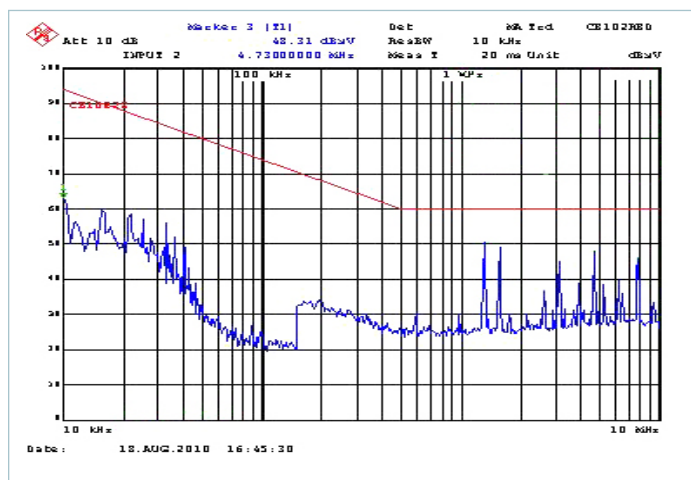
Figure 2 — MIL-STD-461F, CE102; M-FIAM7B and three MIL-COTS PRMs and three MIL-COTS VTMs, 350W
