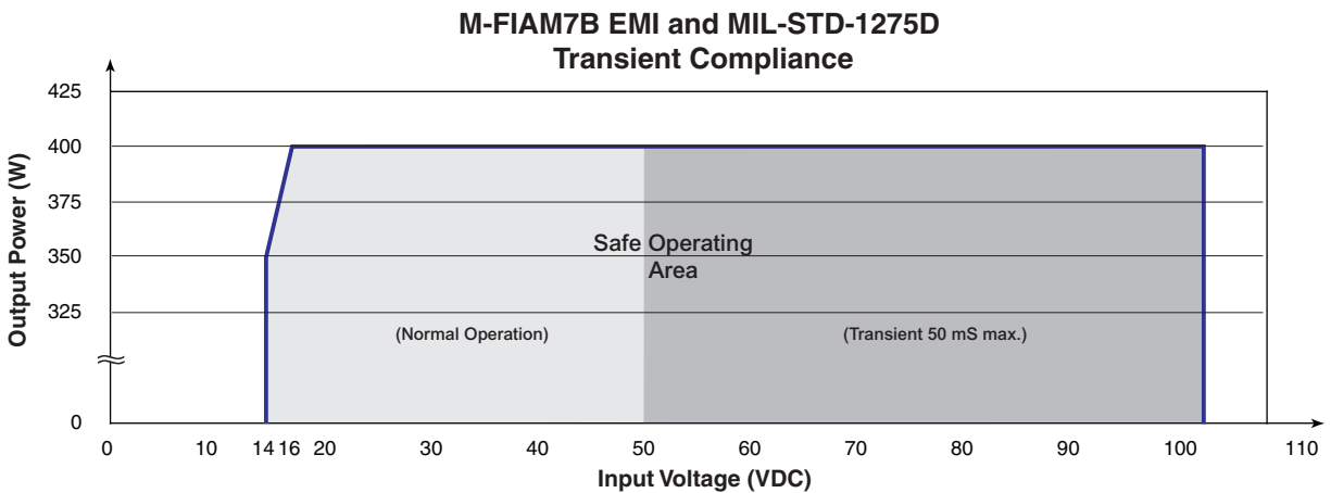
Figure 7 — M-FIAM7B EMI and MIL-STD-1275D transient compliance
