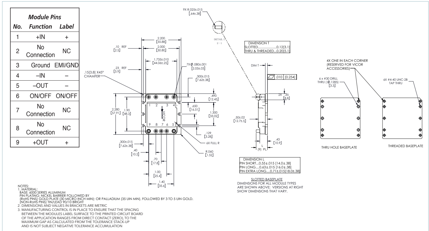
Figure 9 — Mechanical diagram
