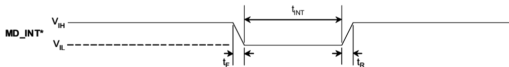
Figure 5-2 Interrupt Timing Diagram
