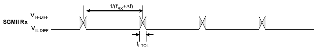
Figure 5-5 SGMII Receive Timing Diagram
