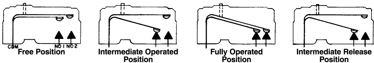
Figure 1. 6BS1-B Sequence of Operation
