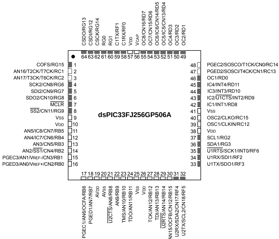
64-Pin QFN (1)
