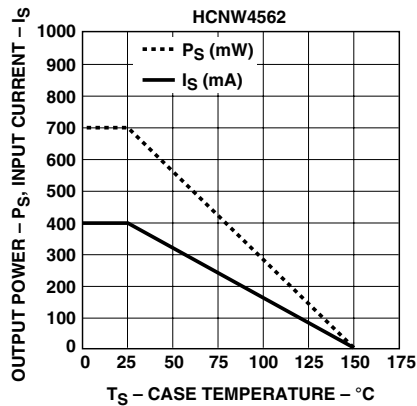
Figure 17. Thermal derating curve, dependence of safety limiting value with case temperature per IEC/EN/DIN EN 60747-5-2
