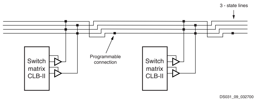
Figure 46: 3-State Buffer Connection to Horizontal Lines
