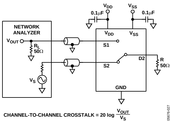
Figure 17. Channel-to-Channel Crosstalk
