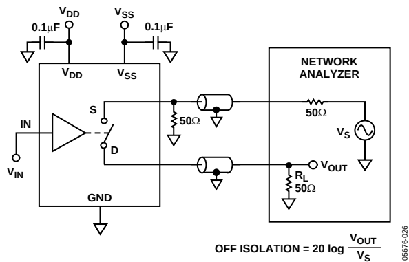
Figure 16. Off Isolation
