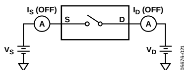
Figure 11. Off Leakage
