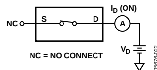
Figure 12. On Leakage
