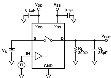
Figure 13. Switching Times
