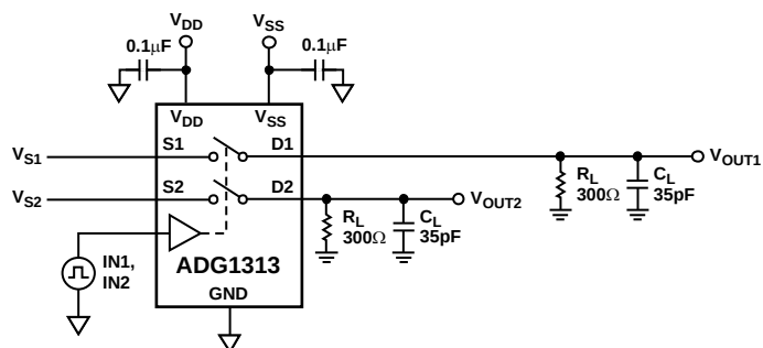
Figure 14. Break-Before-Make Time Delay
