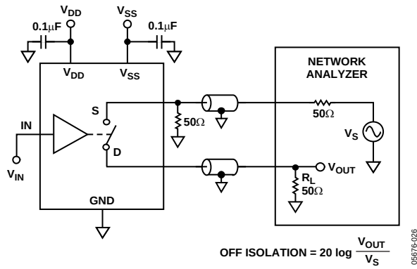
Figure 16. Off Isolation
