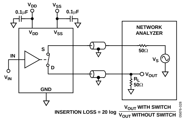
Figure 18. Bandwidth
