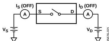
Figure 11. Off Leakage
