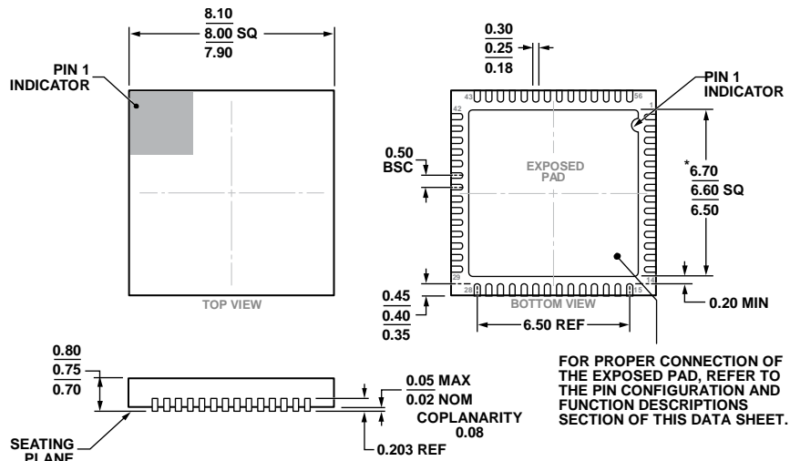
Figure 80. 56-Lead Lead Frame Chip Scale Package [LFCSP_WQ] 8 mm x 8 mm Body, Very Very Thin Quad (CP-56-9)
