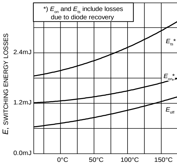
Figure 15. Typical switching energy losses as a function of junction temperature (inductive load, V_{CE}=600\text{V} , V_{GE}=0/15\text{V} , I_C=15\text{A} , R_G=41.8\Omega , Dynamic test circuit in Figure E)
