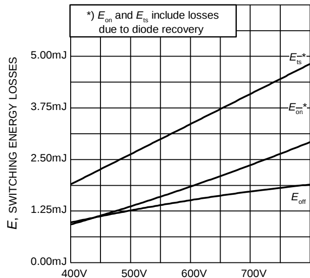
Figure 16. Typical switching energy losses as a function of collector emitter voltage (inductive load, T_J=175^\circ\text{C} , V_{GE}=0/15\text{V} , I_C=15\text{A} , R_G=41.8\Omega , Dynamic test circuit in Figure E)
