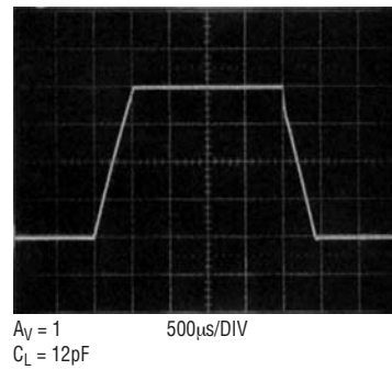
Large-Signal Transient Response V_S = \pm 15V
