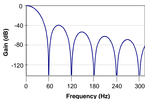
Figure 16. Digital Filter Response (WR = 60 Sps)
