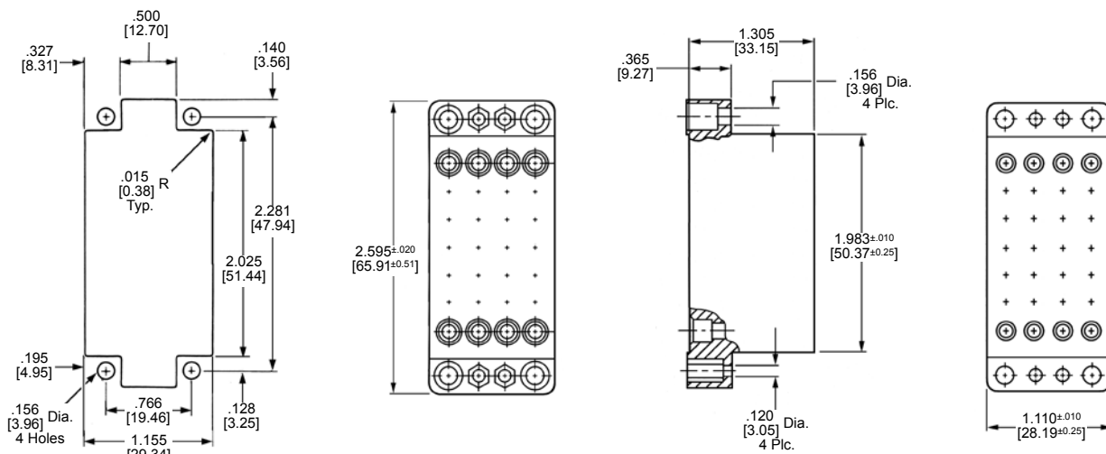
Plug Housing
