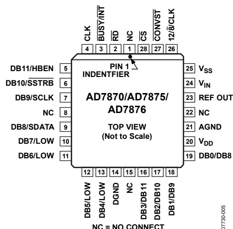
Figure 3. PLCC Pin Configuration
