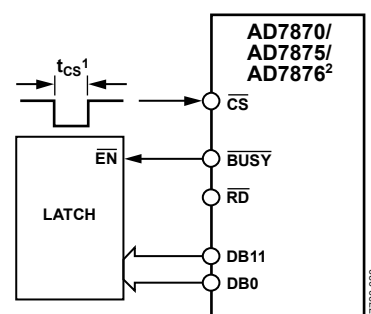
Figure 30. Stand-Alone Operation
