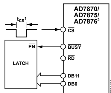
Figure 30. Stand-Alone Operation
