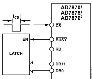
Figure 30. Stand-Alone Operation
