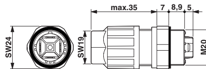
Dimensioned drawing
