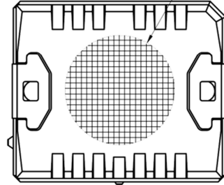
Aspiration area [0,315] ∅ 8
