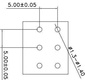
RECOMMEND PCB Layout
