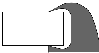
Too much solder Pad geometry too large KKE0071-A-E
