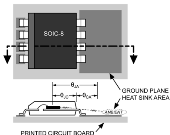
Figure 3. Thermal Resistance
