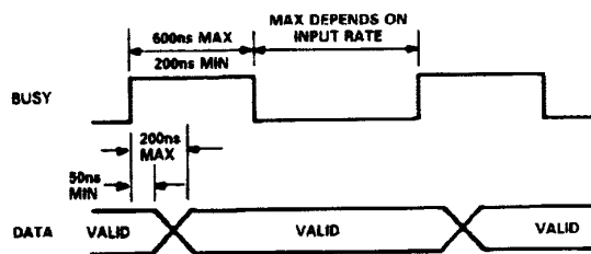
Figure 2. Timing Diagram
