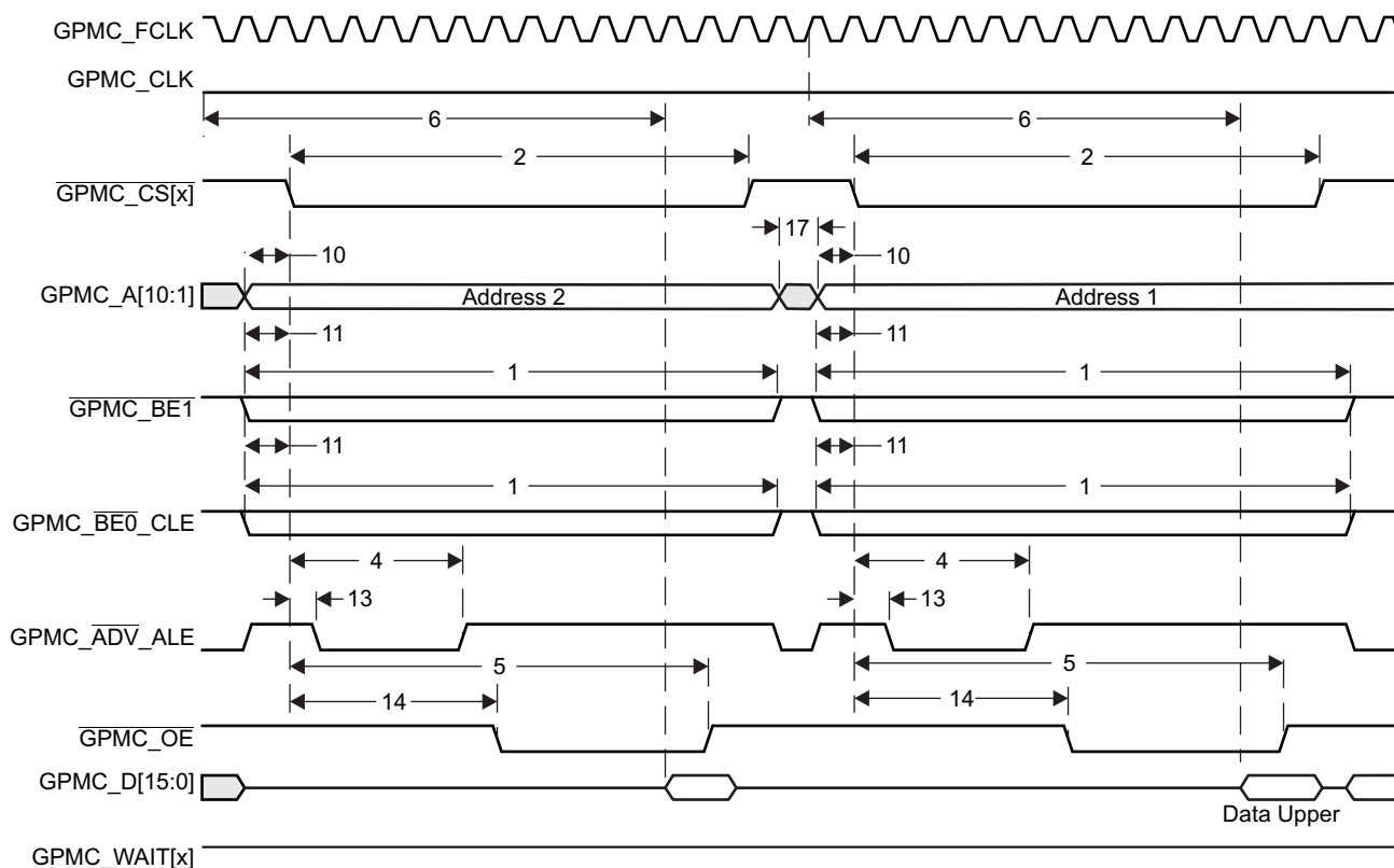
Figure 8-28. GPMC/Non-Multiplexed NOR Flash - Asynchronous Read - 32-Bit Access Timing
