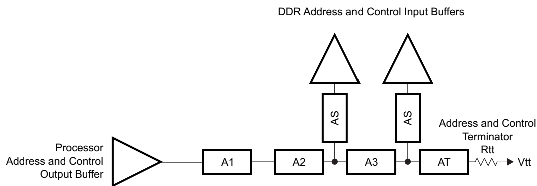
Figure 8-67. ADDR_CTRL Topology for Two DDR3 Devices
