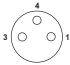
Pin assignment of M8 female connector, 3-pos., view of pin side
