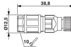
Socket M8 x 1, straight
