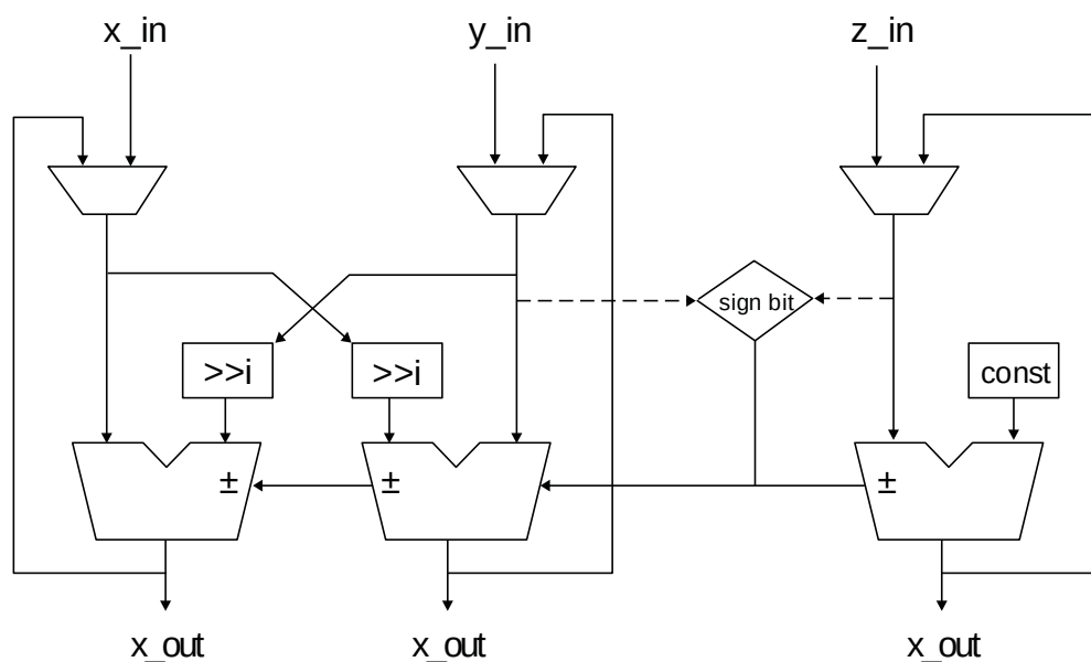
Figure 4.5. Basic CORDIC Arithmetic Unit
