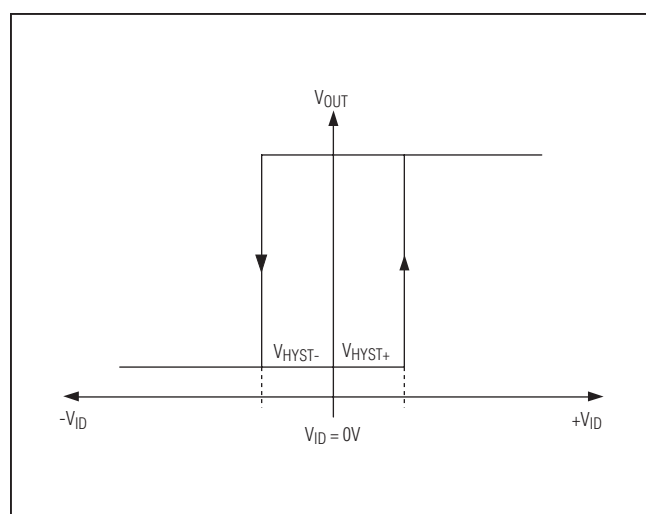
Figure 2. Input Hysteresis
